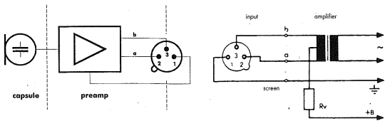
Input circuitry incorporating transformer without center tap (ungrounded).
